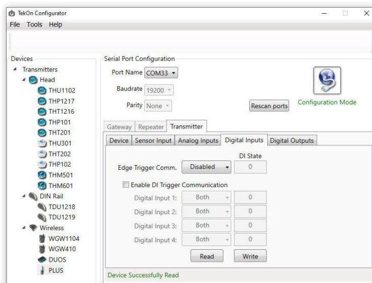
Figure 26 - Digital inputs tab in Tekon Configurator software
