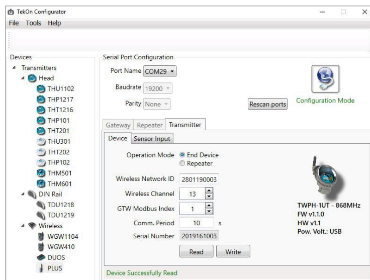
Figure 13 - Device tab in Tekon Configurator software
