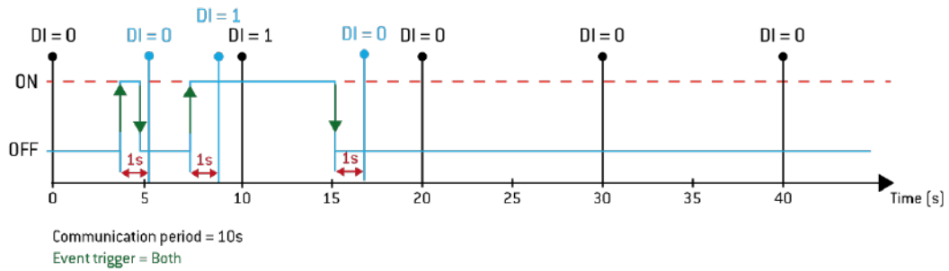
Figure 31 - Behaviour of digital input activation by Both
