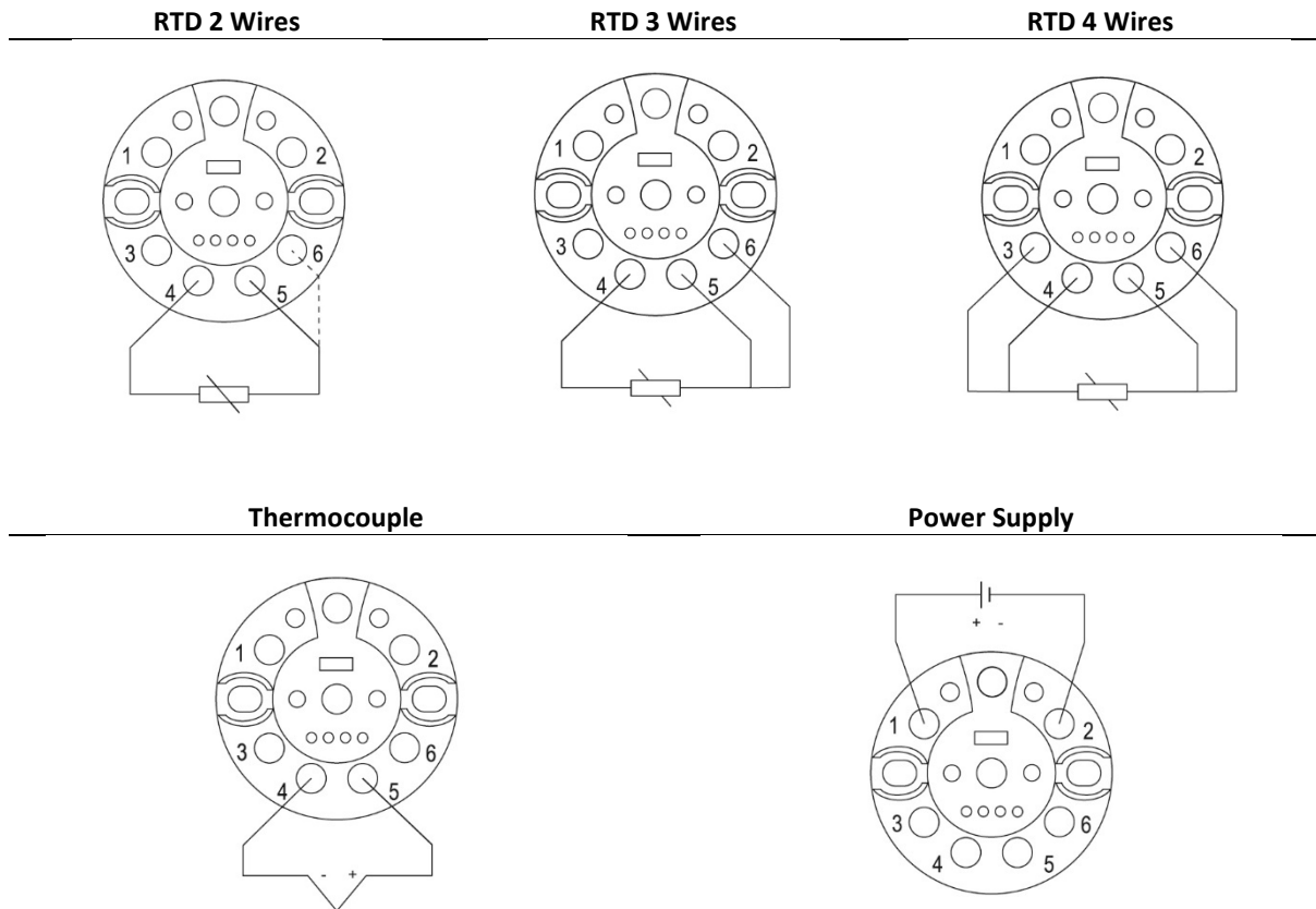
Figure 15 - TWPB-1UT wire connections
