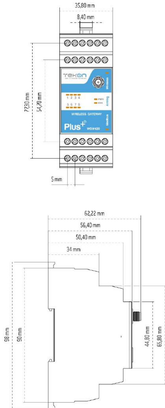
Figure 39 – WG420 gateway mechanical interface and dimensions
