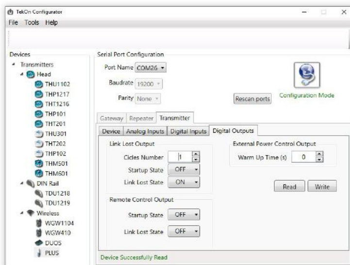
Figure 9 - Digital outputs tab in Tekon Configurator software
