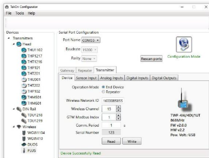
Figure 22 - Device tab in Tekon Configurator software
