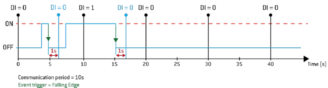
Figure 29 - Behaviour of digital input activation by Falling Edge
