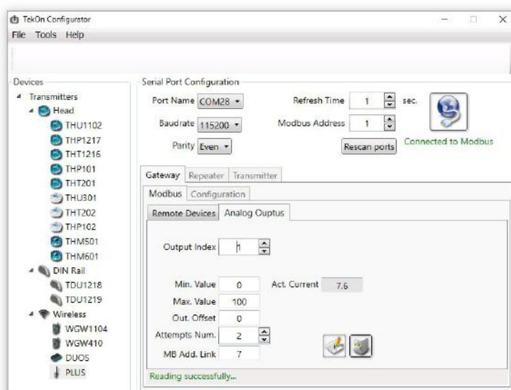
Figure 46 - Tekon Configurator layout of analog outputs tab
