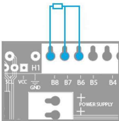
Figure 20 - PT100 connection
