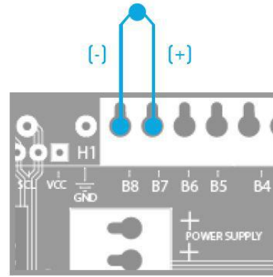
Figure 21 - Thermocouple connection
