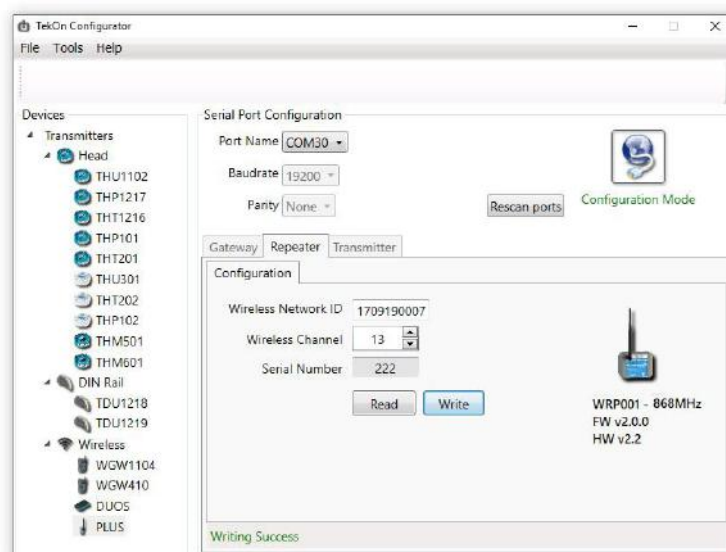
Figure 37 - Configuration of WRP001 repeater at Tekon Configurator software
