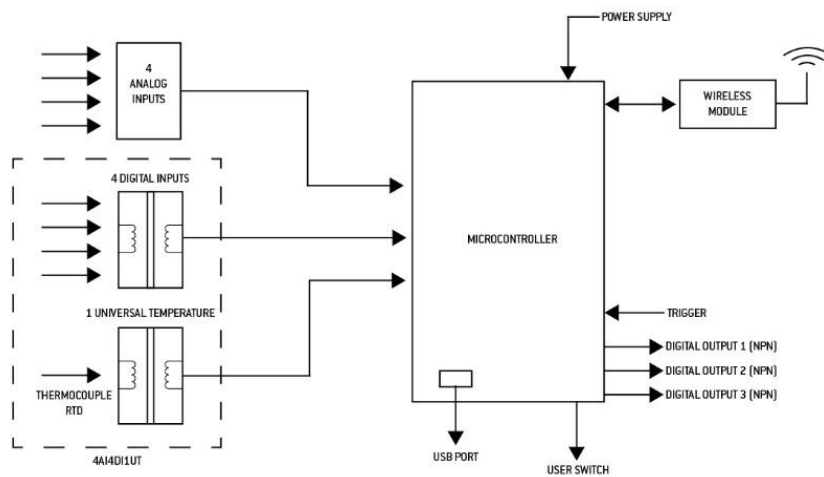
Figure 17 - Block diagram of TWP-4AI4DI1UT
