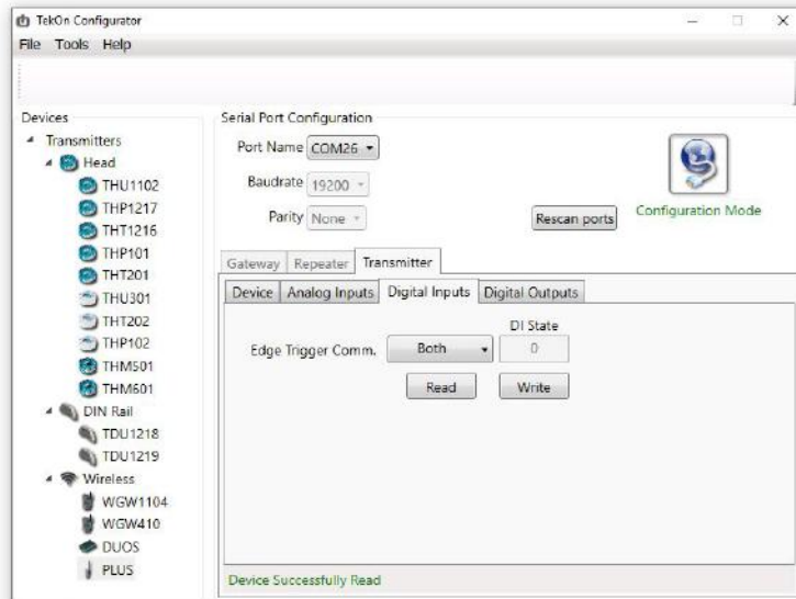
Figure 7 - Digital input tab in Tekon Configurator software
