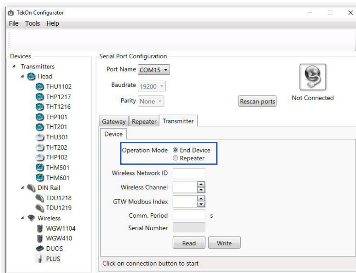
Figure 47 - Transmitter operation mode configuration in Tekon Configurator
