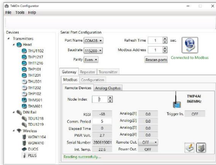
Figure 43 - Tekon Configurator layout of remote devices tab
