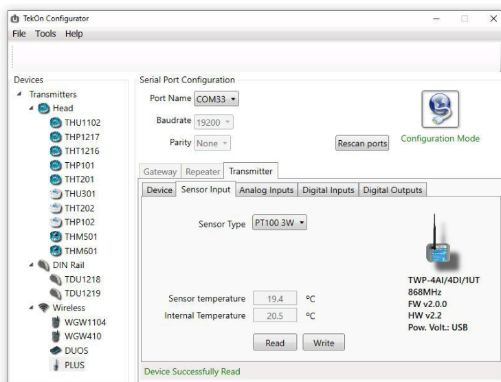
Figure 23 - Sensor input tab in Tekon Configurator software
