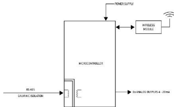
Figure 40 - Block diagram of WGW420 gateway
