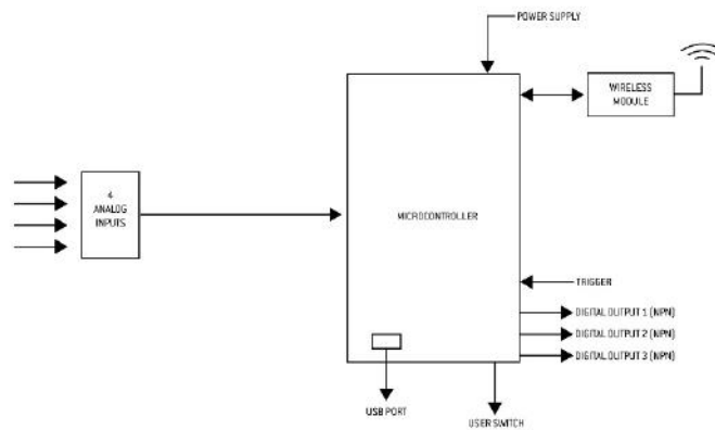
Figure 2 - Block diagram of TWP4AI transmitter
