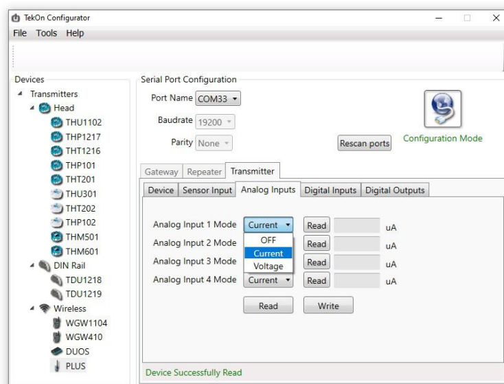
Figure 25 - Analog inputs options in Tekon Configurator software
