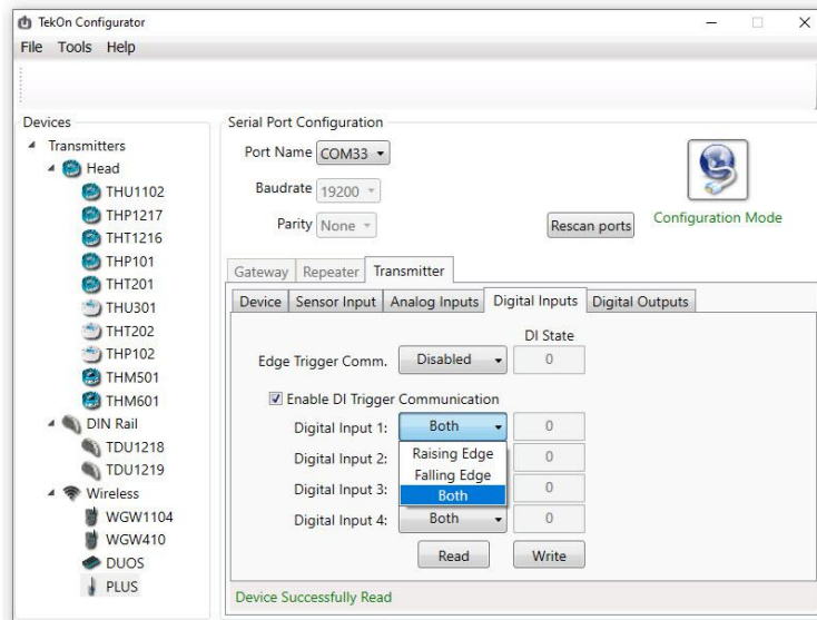
Figure 28 - Digital Inputs configuration and options
