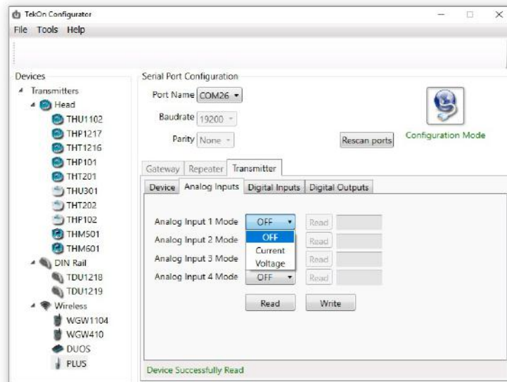
Figure 6 - Analog inputs options in Tekon Configurator software
